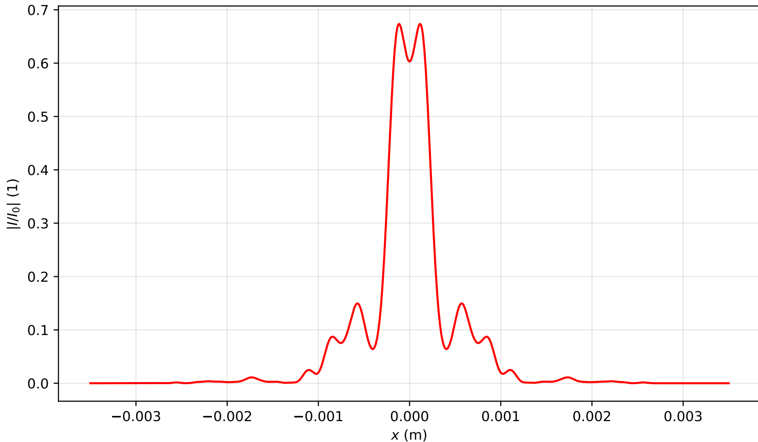
Intensity profile I(x, y = 0, z = 1.433)/I_0 , \text{Pin}=7.5\text{Pcr} , artificial time
